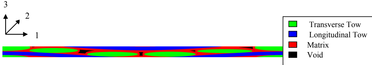
Figure 3.—2D Unit cell of 5HS composite.
